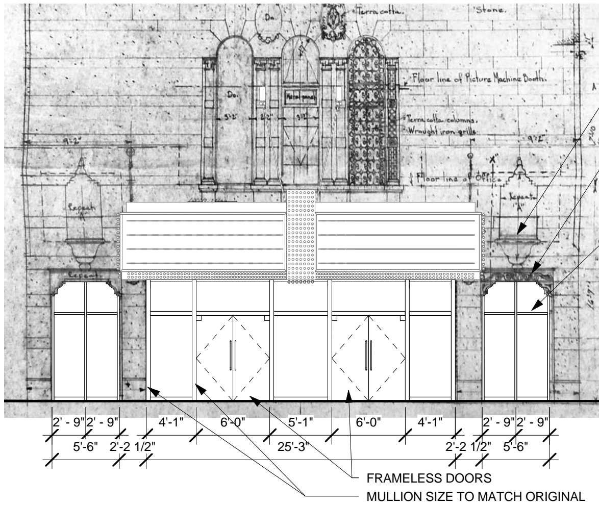
A2 NEW ENTRY FENESTRATION - PREFERRED 1/8" = 1'-0"
