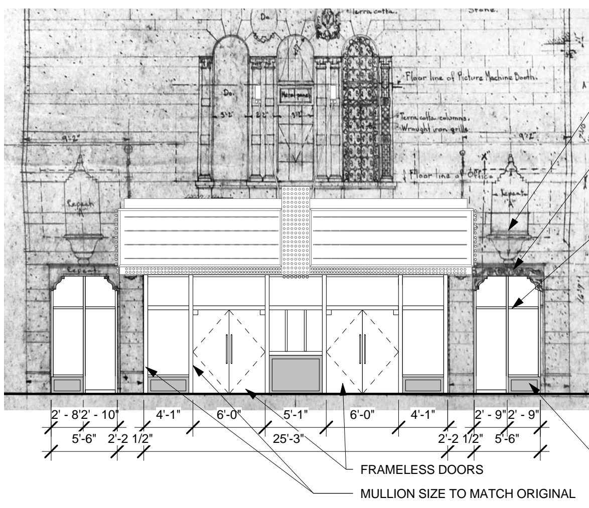
A1 NEW ENTRY FENESTRATION - ALTERNATE 1/8" = 1'-0"
