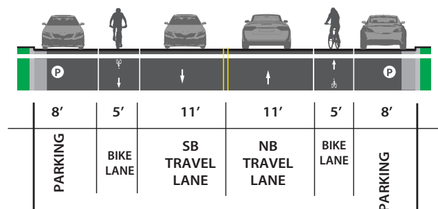
Typical proposed cross section
