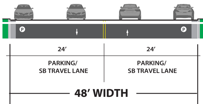
Typical existing cross section
